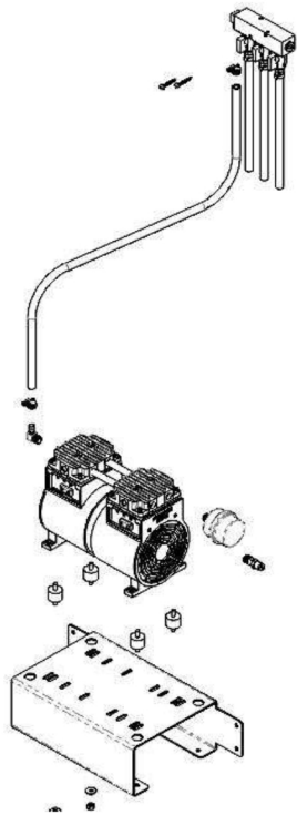
KM-120, ½ HP Compressor
