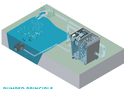
PUMPED PRINCIPLE
