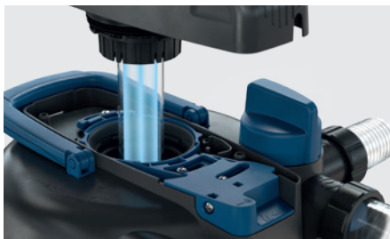
Easy to replace the lamp: The UV housing can be easily removed during operation for replacing the integrated UV lamp.
