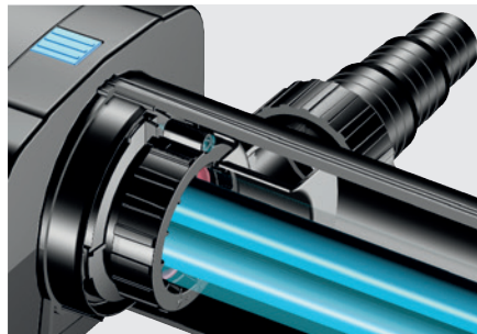
UVC lamps in the glass tube: The use of high-quality UVC lamps guarantees a long service life and consistently good irradiation performance.
