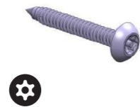
Security Screw 4.8x30mm Material: Steel BZP ICQ4627S
