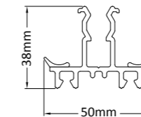
Rafter Thermal Core Material: Extruded uPVC ICQ4011W - White
