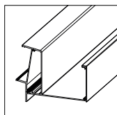
02. Gutter profile
