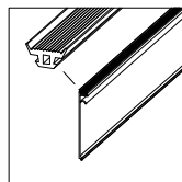
14. Trim click strip
